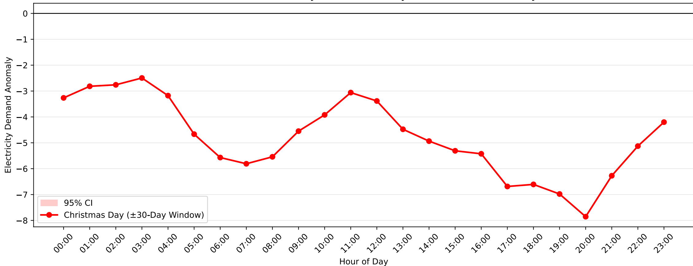
Pennant Hills Demand Anomaly: Christmas Day (2016–2017, \pm 30 -Day Window)
