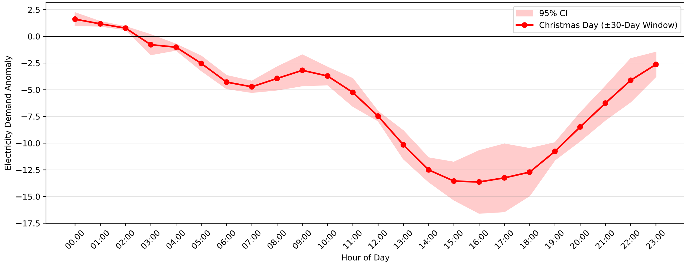
Pennant Hills Demand Anomaly: Christmas Day (2007–2008, \pm 30 -Day Window)
