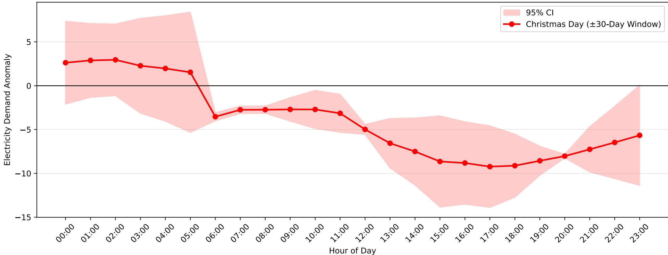
Pennant Hills Demand Anomaly: Christmas Day (2014-2015, \pm 30 -Day Window)
