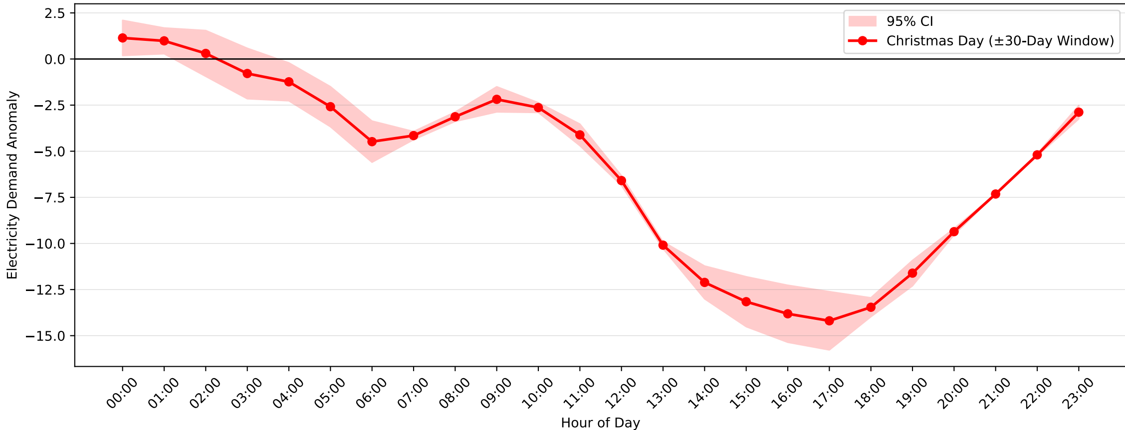
Pennant Hills Demand Anomaly: Christmas Day (2006–2007, \pm 30 -Day Window)
