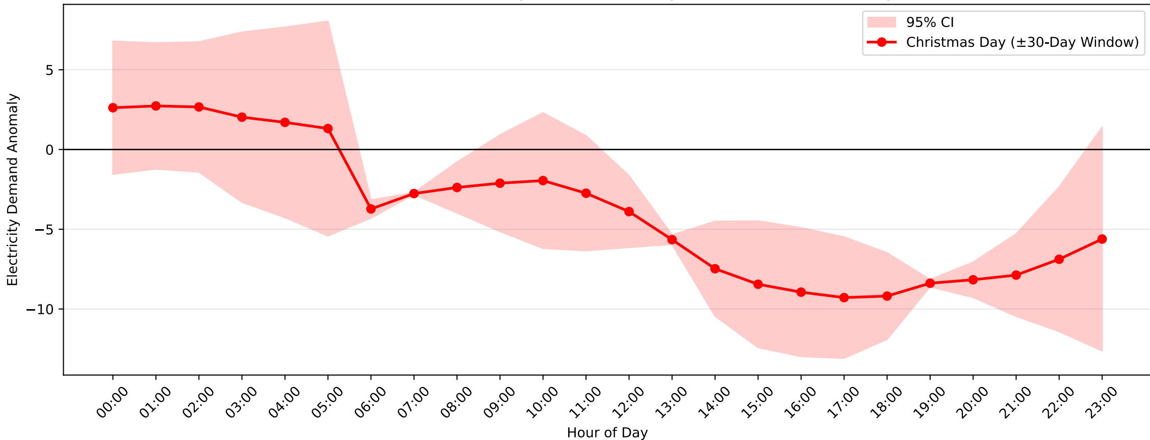
Pennant Hills Demand Anomaly: Christmas Day (2013-2014, \pm 30 -Day Window)
